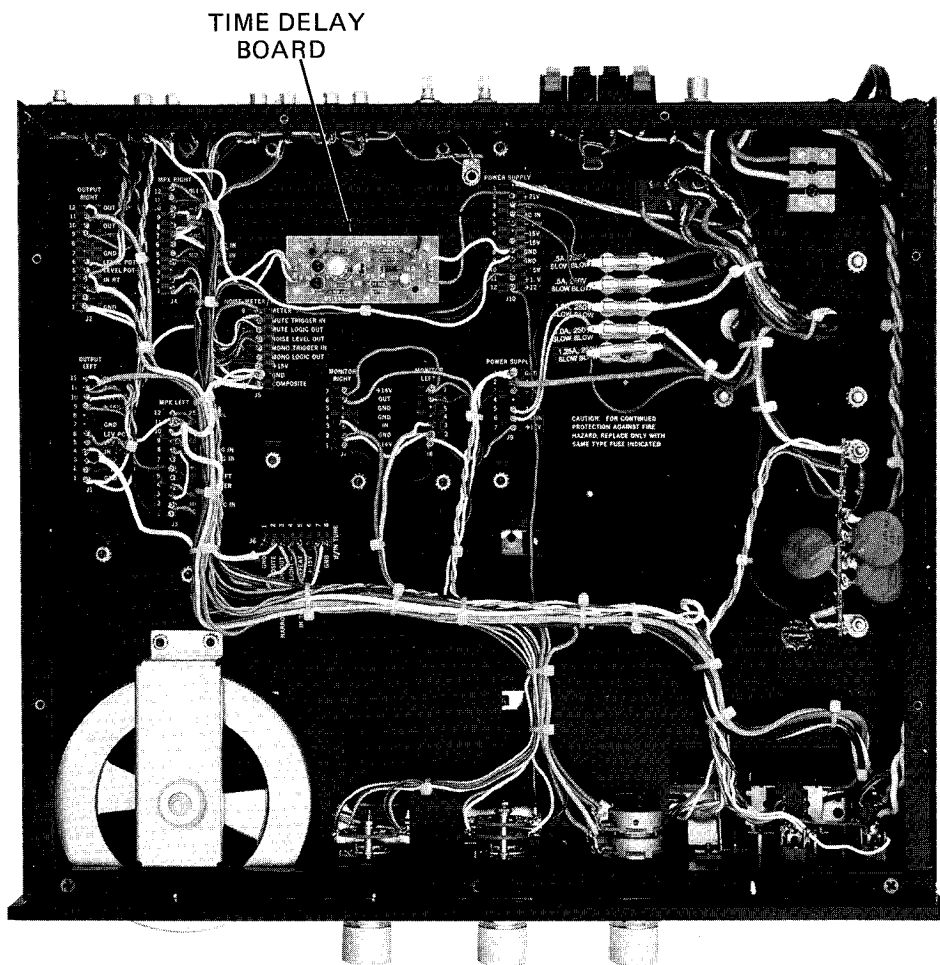
BOTTOM VIEW
