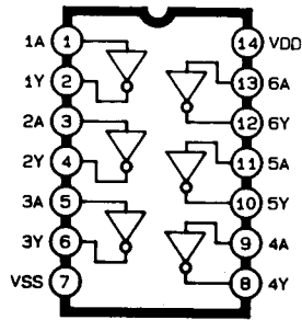
IC1 : TC4069BP Tone Amp.
