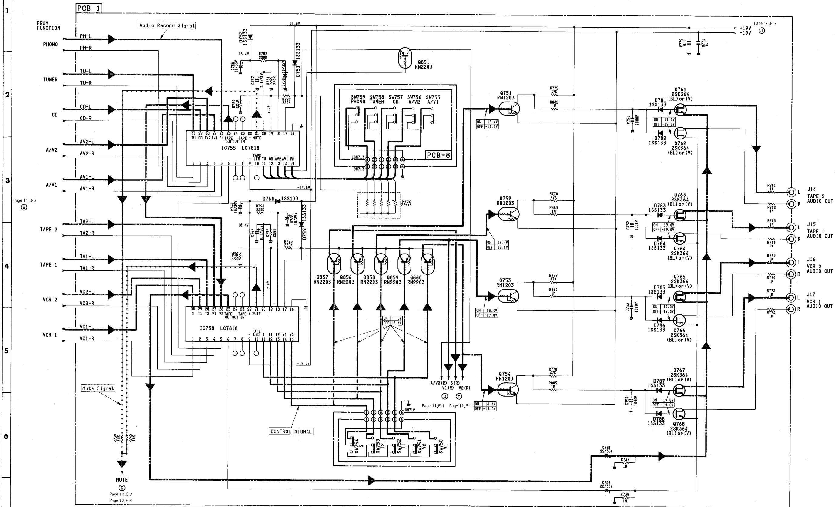
SCHEMATIC DIAGRAM (3)
